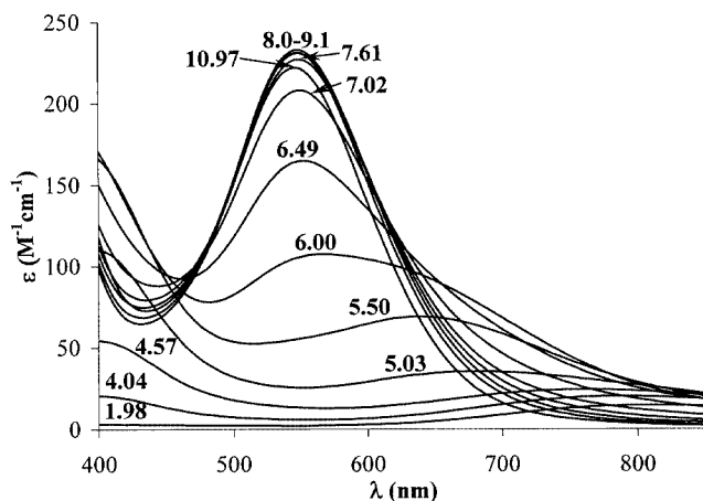
Figure 3. Visible absorption spectra of the \text{Cu}^{\text{II}} -SalGly-L-Ala system at a 1:2 metal ion to ligand ratio at several pH values and c_{\text{Cu}} = 0.006 \text{ M}
